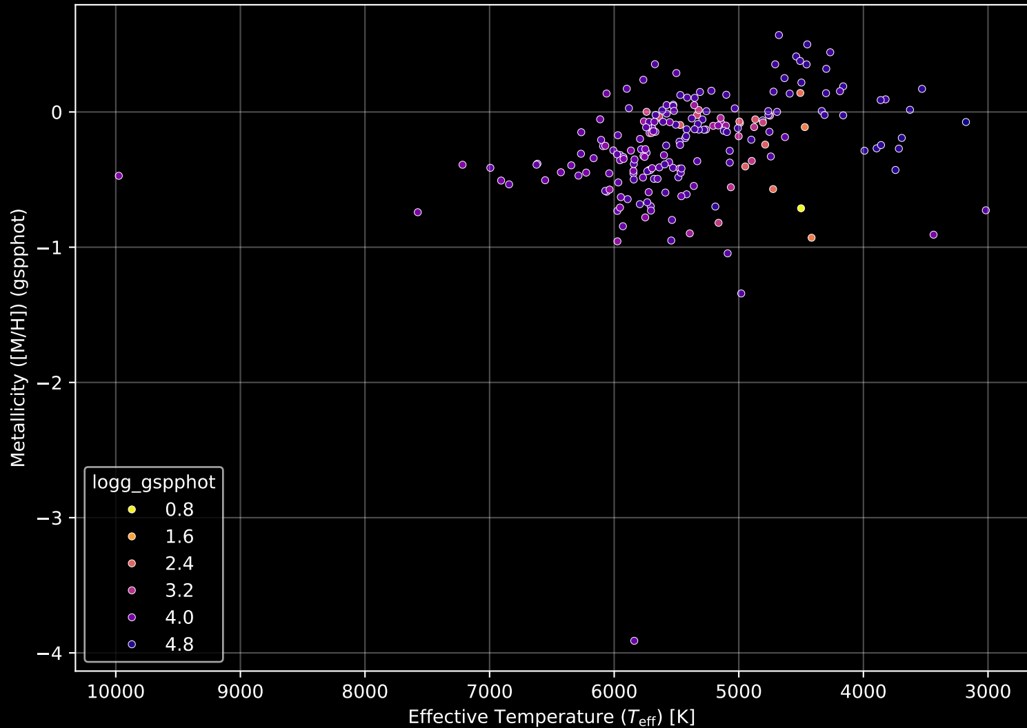
APOGEE DR17 Field: [146-46_MGA] Stellar Population Parameters (n= 204)
