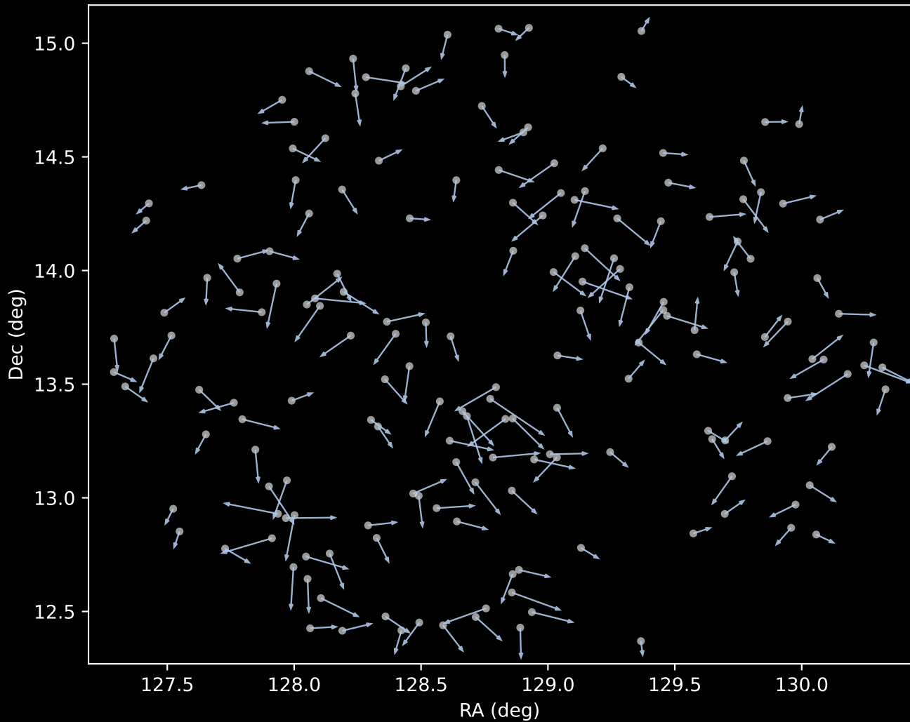
APOGEE DR17 Cluster 1 Proper Motion Vectors (n=177)
