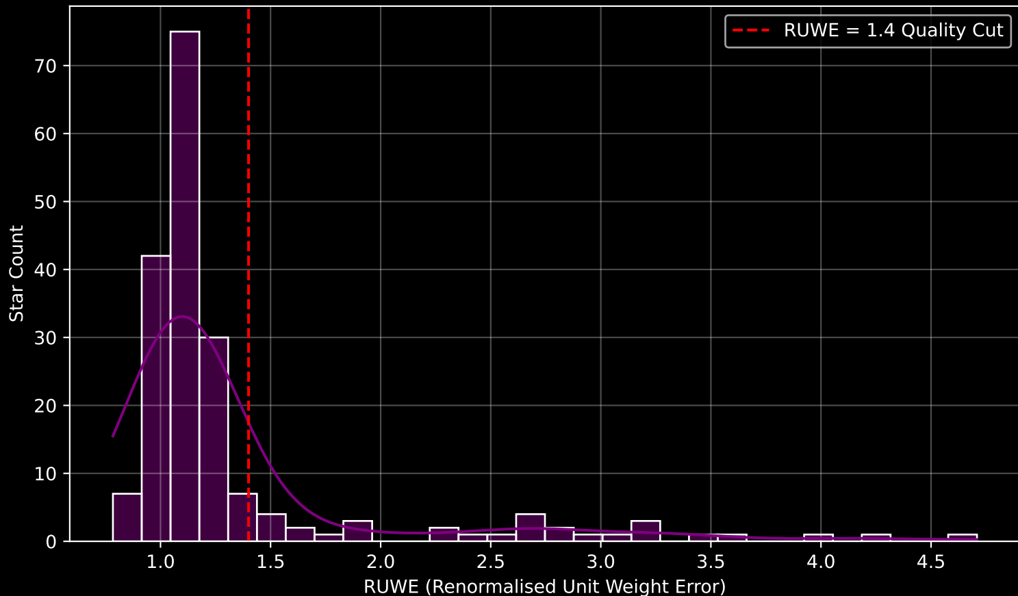
GAPOGEE DR17 Field [146-46_MGA] RUWE Distribution (n= 191)
