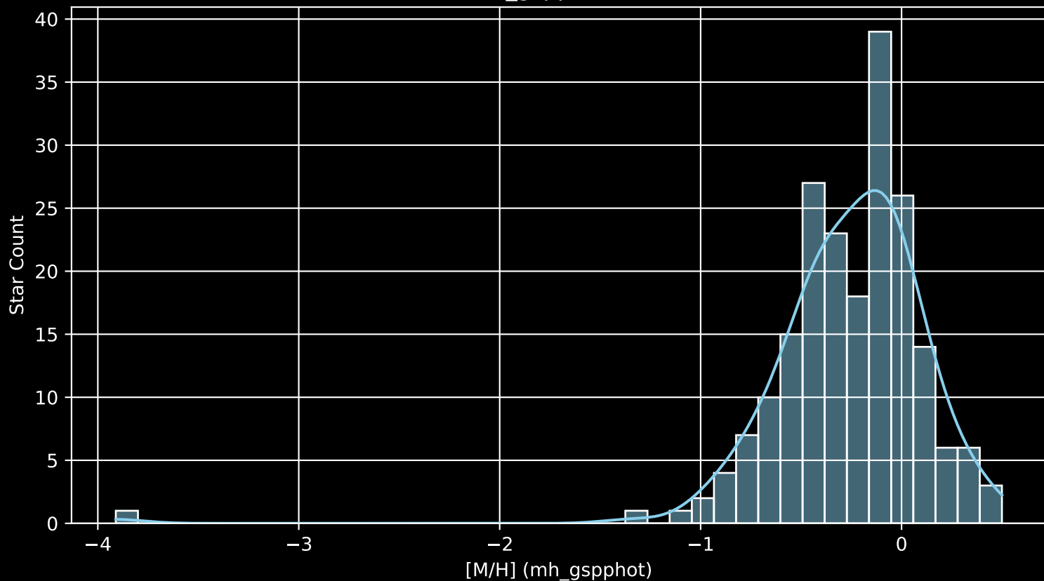
APOGEE DR17 Field: [146-46_MGA [M/H] (mh_gspphot) (n= 203)
