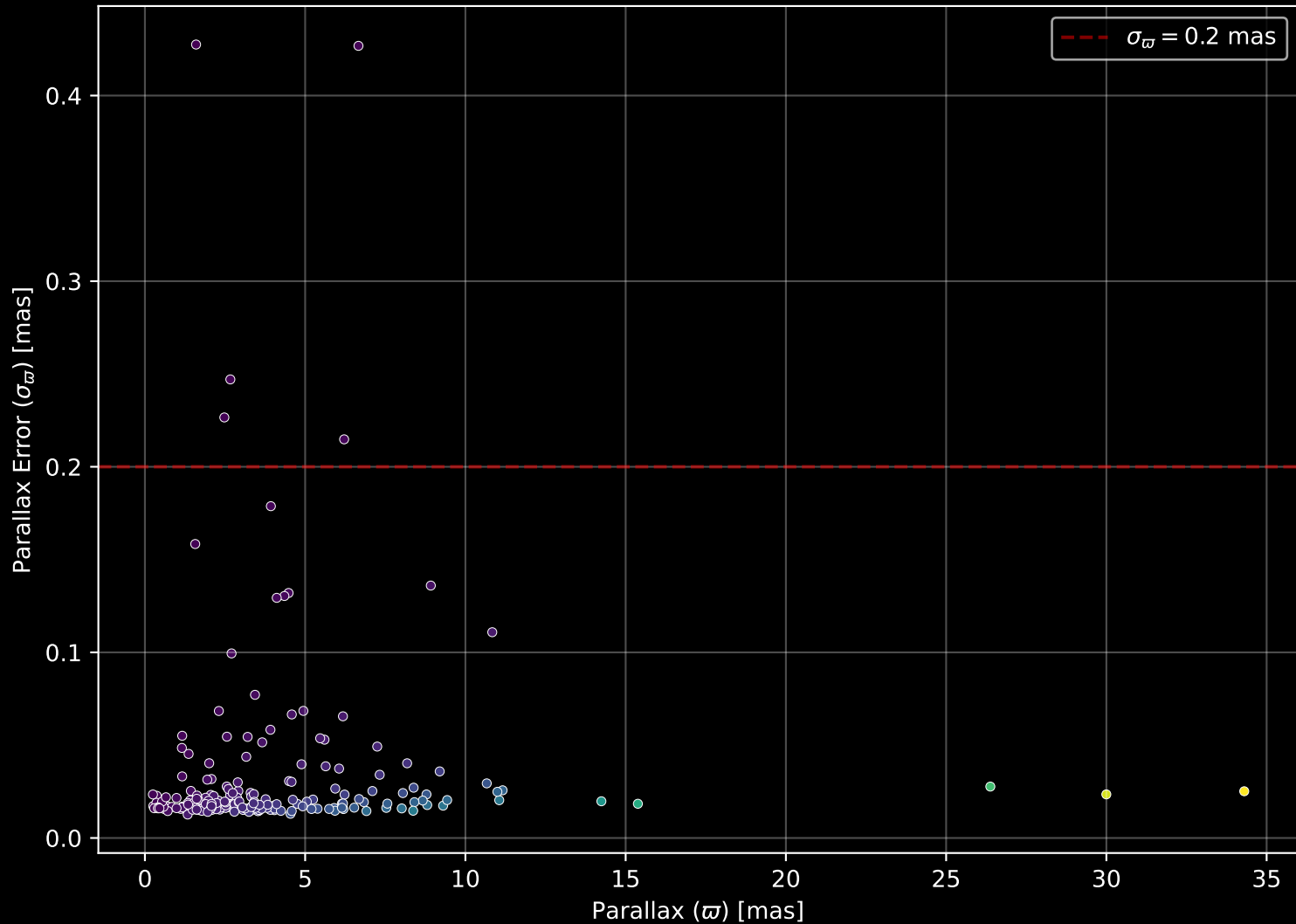
APOGEE DR17 Field: [146-46_MGA] Parallax Quality (n= 204)
