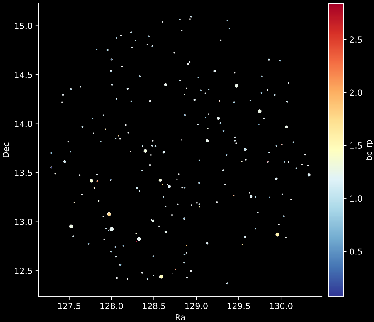
APOGEE DR17 Field: [146-46_MGA] Stars: 204
