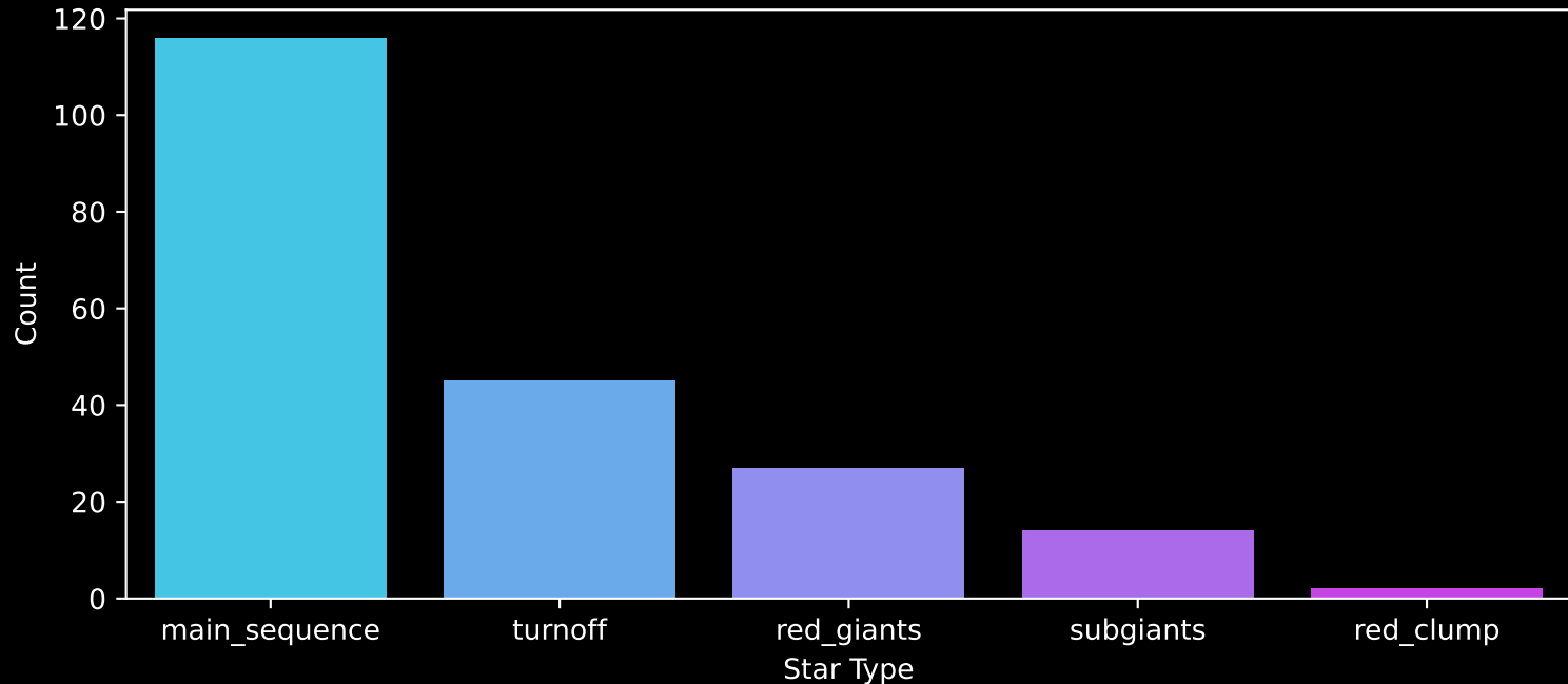
APOGEE DR17 Field: [146-46_MGA] Count plot of Star Type
